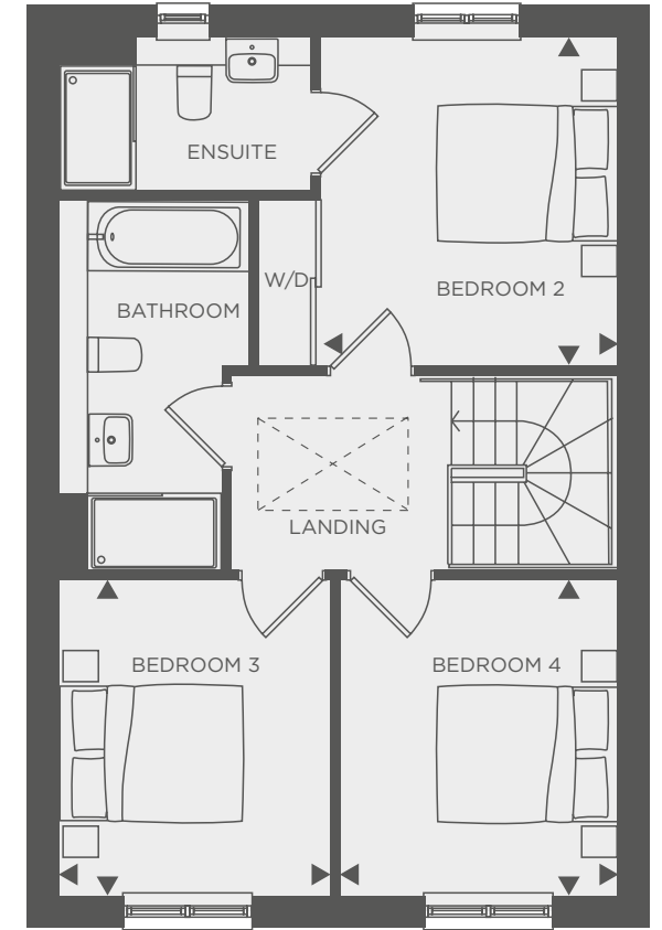
SECOND FLOOR
